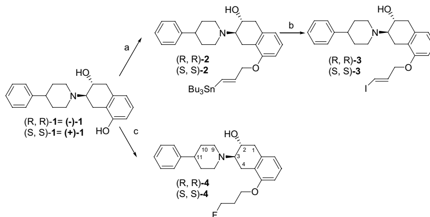
Scheme 1. Synthesis of the enantiomeric pairs (R,R) / (S,S) -5-AOIBV, 3 and (R,R) / (S,S) -5-FPOBV, 4 . Reagents and conditions: (a) TBAOH, \text{CH}_3\text{CN} , (E)\text{-Bu}_3\text{SnCH=CH-CH}_2\text{OTs} , 80^\circ\text{C} ; (b) from (S,S) -2: \text{I}_2 , \text{CHCl}_3 , rt, from (R,R) -2: NIS, THF, rt; (c) TBAOH, \text{CH}_3\text{CN} , \text{F}(\text{CH}_2)_3\text{OTs} , 80^\circ\text{C} .
