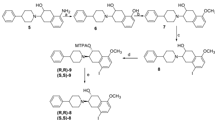
Scheme 2. Synthesis of the enantiomeric pair (R,R) - and (S,S) -8-MOIBV, 8 . Reagents and conditions: (a) \text{NaNO}_2 , \text{H}_2\text{SO}_4 , THF, 0^\circ\text{C} then reflux; (b) TBAOH, \text{CH}_3\text{CN} , \text{CH}_3\text{I} , 80^\circ\text{C} ; (c) \text{ICl} , \text{CH}_3\text{CO}_2\text{H} , rt; (d) (R) -MTPA-Cl, 4-DMAP, TEA, \text{CHCl}_3 , rt; (e) 2N NaOH, \text{CH}_3\text{OH} , THF, rt.
